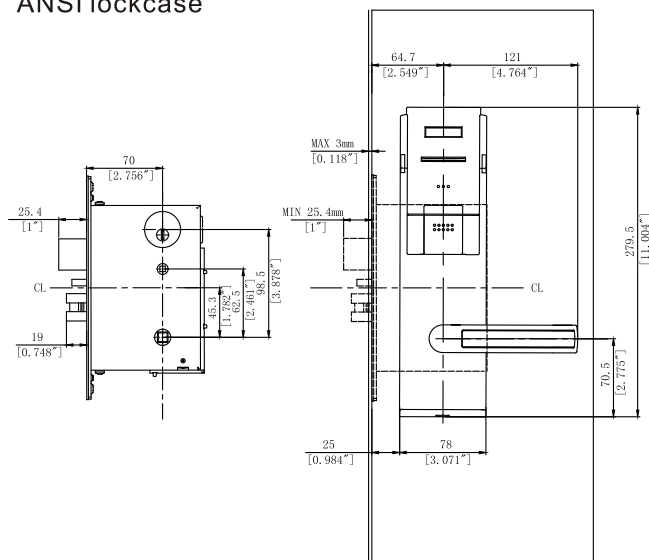
ANSI lockcase
